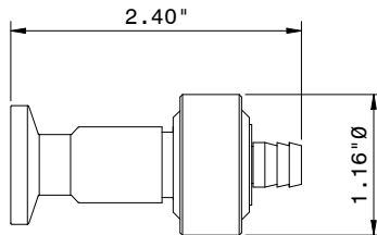
IN-LINE 1/2" FERRULE P/N OFSVILF
