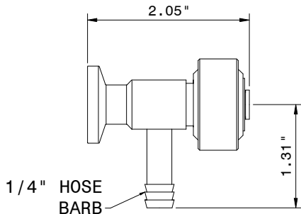
90° 1/2" FERRULE P/N OFSV90F
