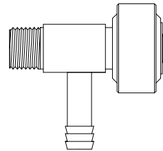
90° 1/4" NPT P/N OFSV90N
